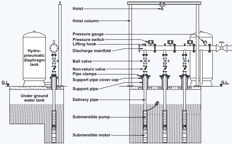
FIG. 4 SYSTEM COMPONENTS
